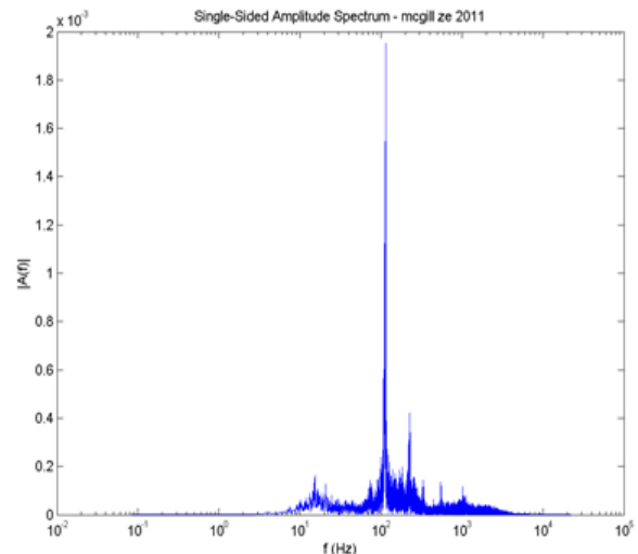
Figure 6 - Spectral Analysis of MEST's 2011 Sound Results
