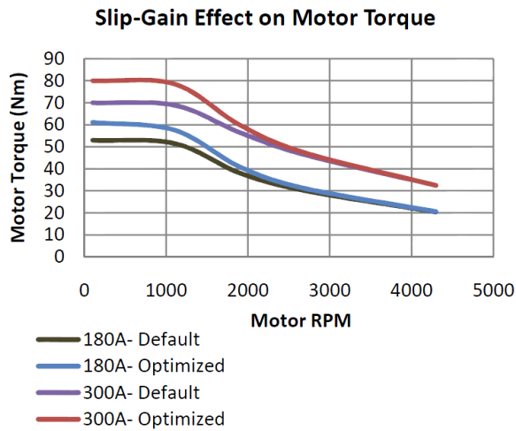
Graph 3 – Motor torque versus RPM
