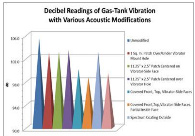
Figure 9 - Decibel Reading Results for Various Modifications
