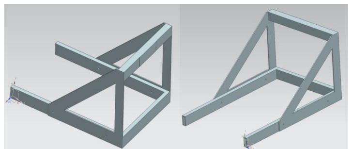
Figure 5 – 2012 Hitch design using NX Unigraphics 7.5
