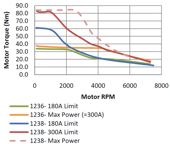
Graph 2 – Motor torque versus RPM
